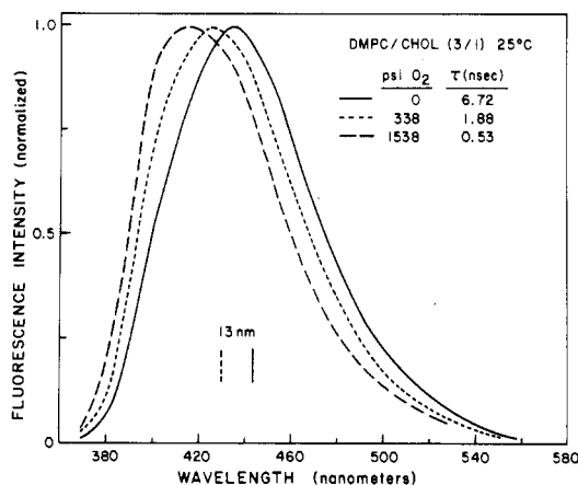
FIGURE 3: Effects of oxygen quenching on fluorescence emission spectra of TNS-labeled DMPC/Chol (3:1) vesicles. The vertical solid and dotted lines illustrate \nu_{cg}^{-1} , in nanometers, in the absence and presence of oxygen, respectively. The fluorescence lifetimes at each oxygen pressure are shown on the figure.
